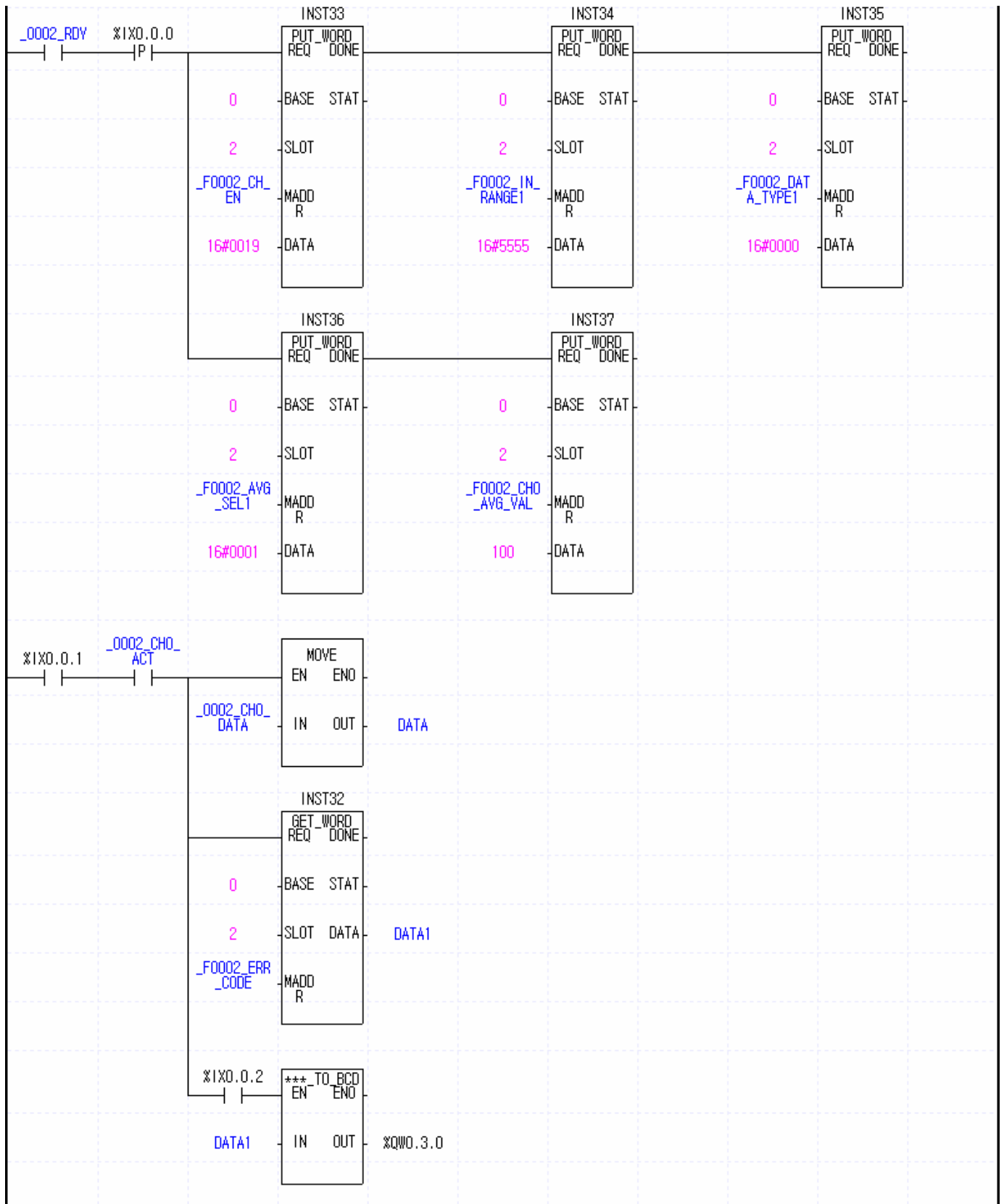
(b) Program example using PUT/GET instruction
