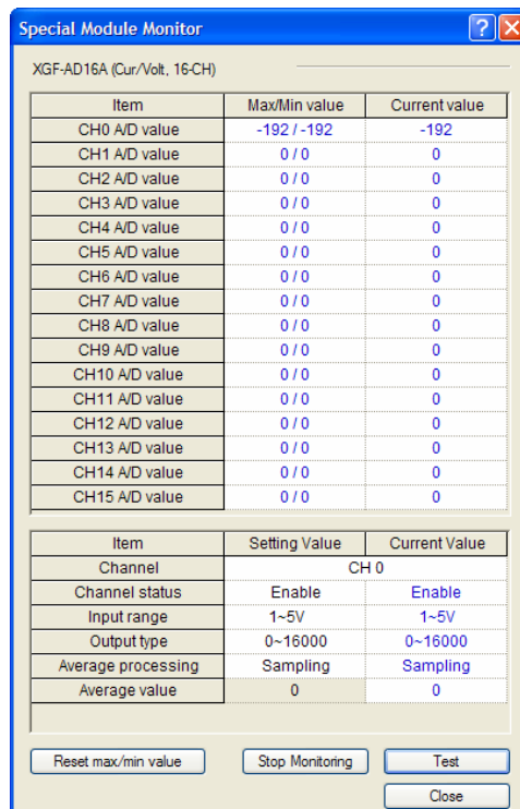
[Fig. 5. 6] Execution screen of [Reset max./min. value]
