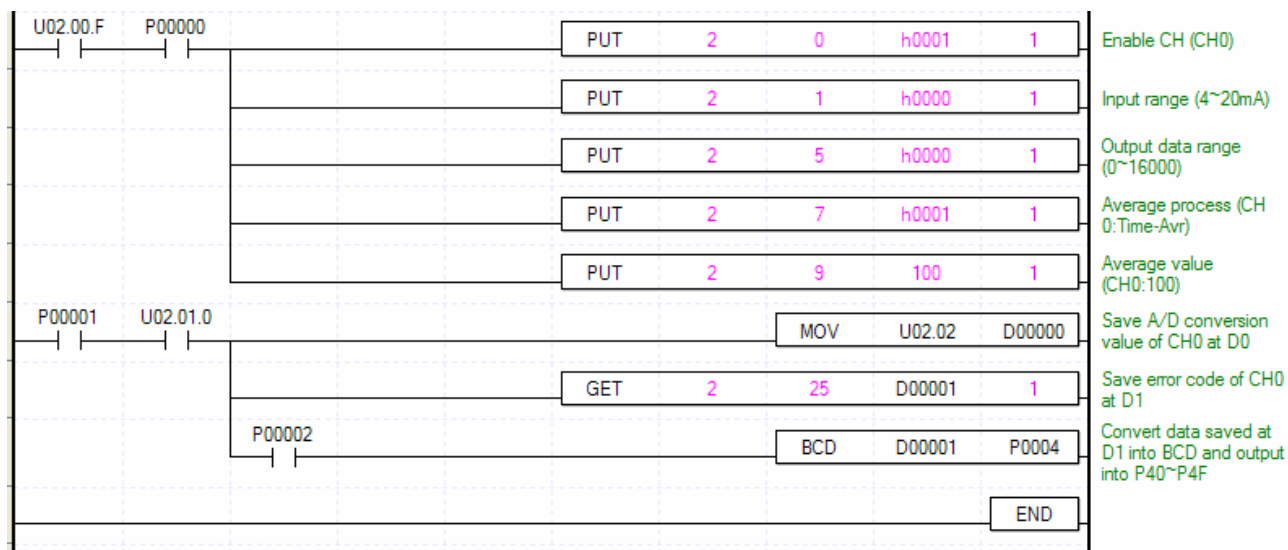
(b) Program example using PUT/GET instruction
