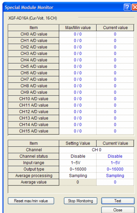
[Fig. 5. 4] Execution screen of [Start Monitoring]
