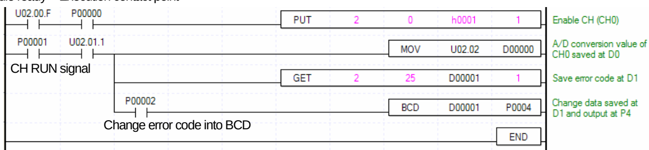
(b) Program example using PUT/GET instruction
