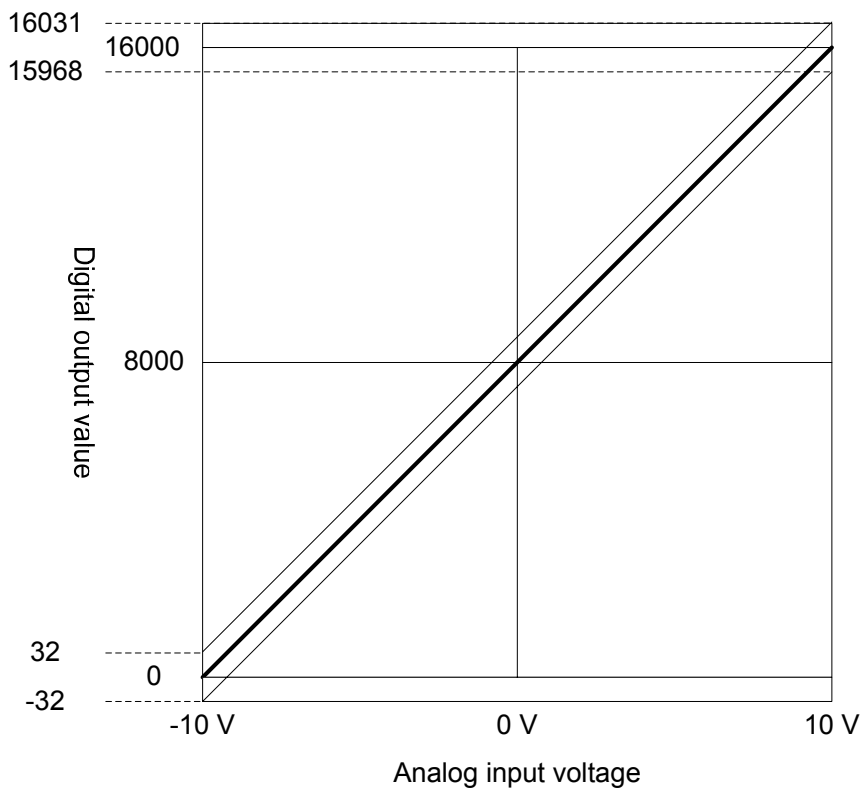
[Figure 2.1] Accuracy (in case of 25 \pm 5^\circ\text{C} )
