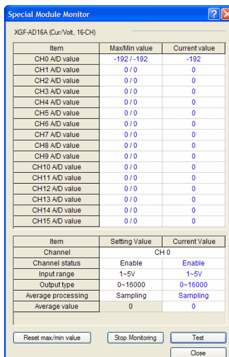
[Fig. 5. 5] Execution screen of [Test]
