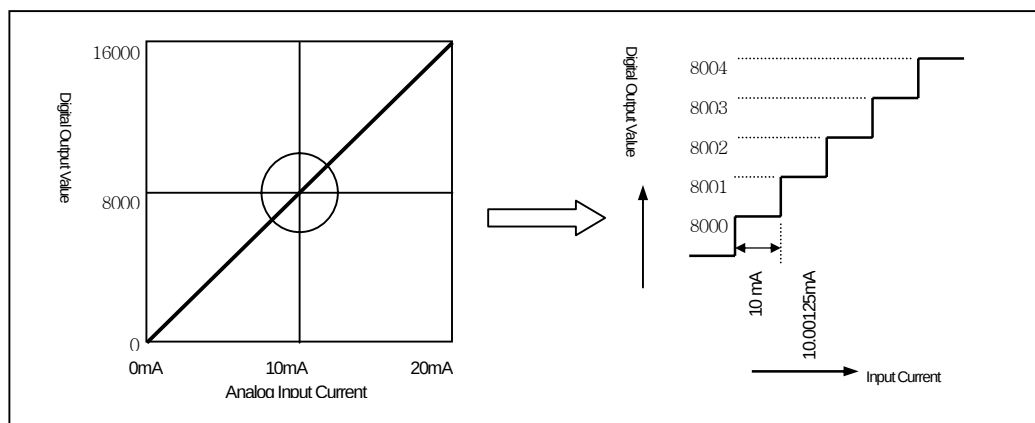
[Fig. 1.6] Characteristics of A/D conversion (Current Input)
