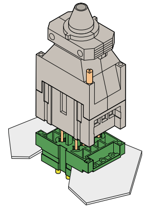
Reverse mounting
