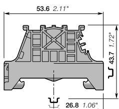
BAM4
