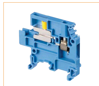
Neutral disconnect: screw clamp terminal blocks
