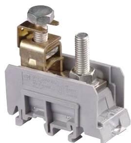
M70/31.AF
