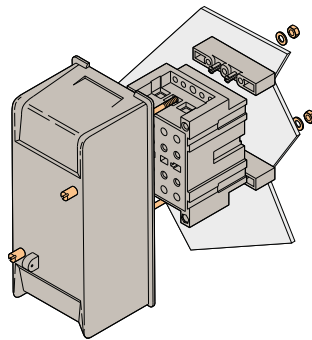
Base mounting
